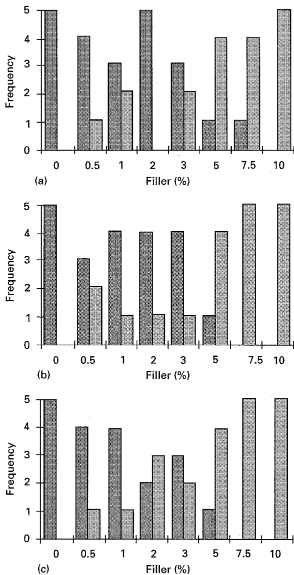
Figure 6 Histogram illustrating the distribution between (■) ductile and (□) brittle failures in the mechanical tests of dried PCD (a), PCA (b) and dried PBT (c).
